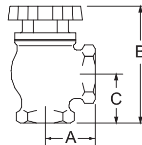
35XL (3/4" - 2")
